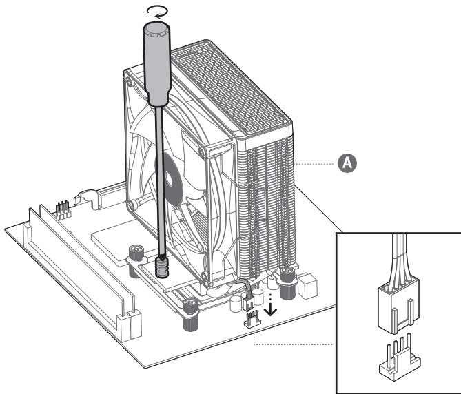
4-PIN/CPU_FAN/CPU_OPT
