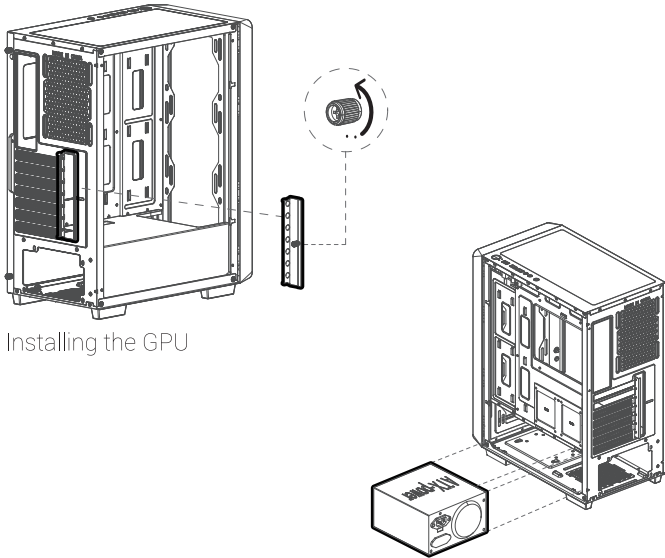
Installing the Power supply
