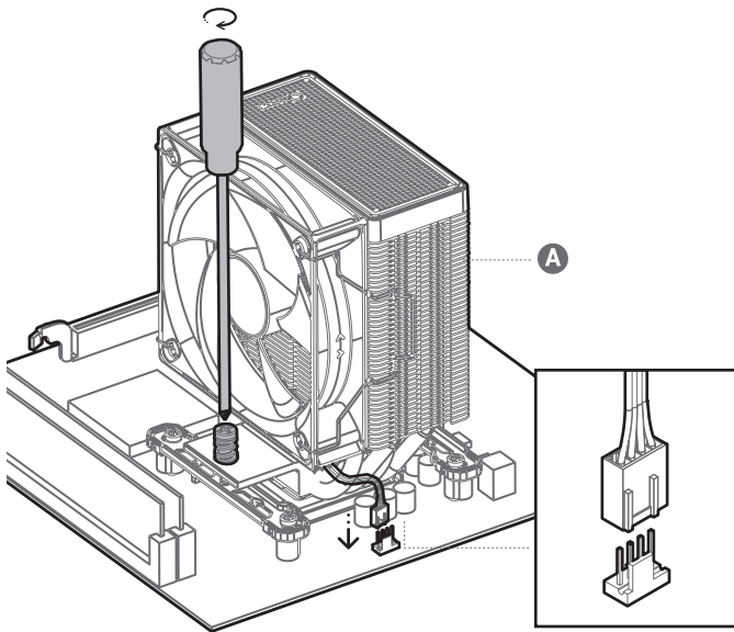
4-PIN/CPU_FAN/CPU_OPT
